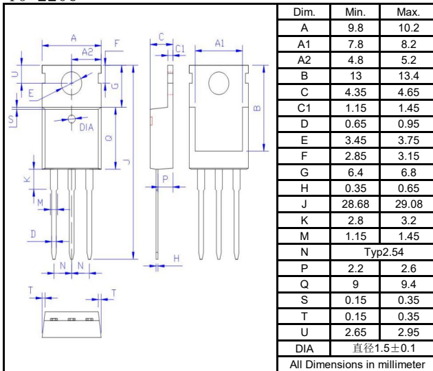
T0-220C
